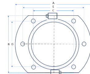
Mounting Flange Detail
