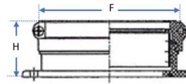
Mounting Flange Elevation
